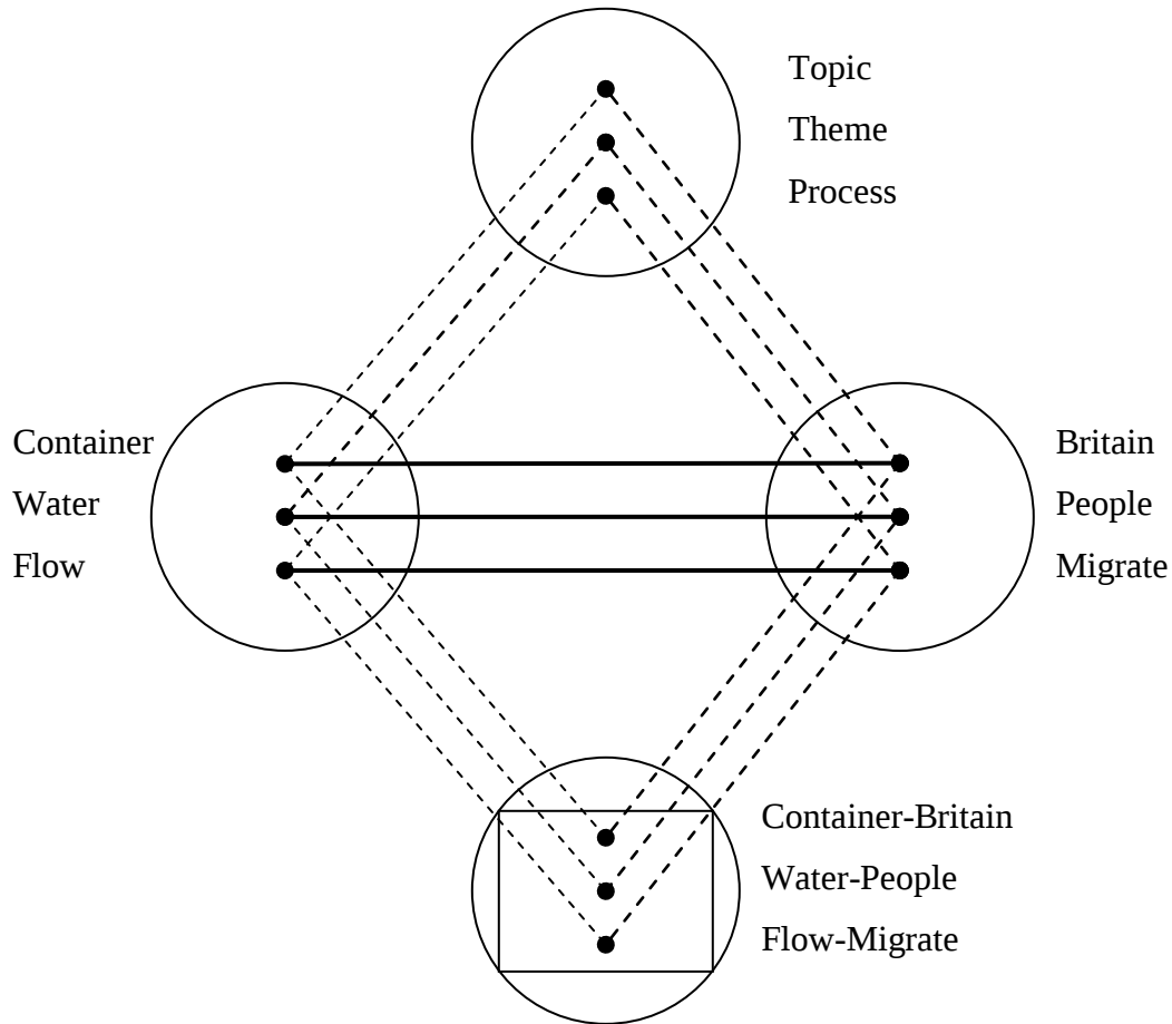
Figure 5. Conceptual blending network for interaction of ‘flow of immigration’ and ‘Britain is full up’
